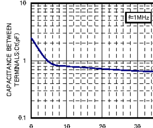
VR-Ct CHARACTERISTICS
